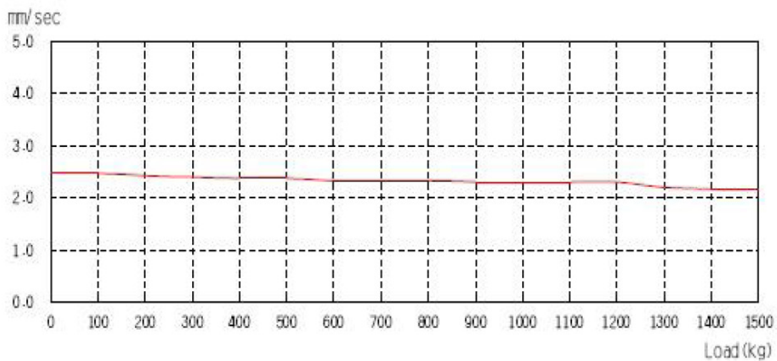
Speed (mm/sec) vs Load
